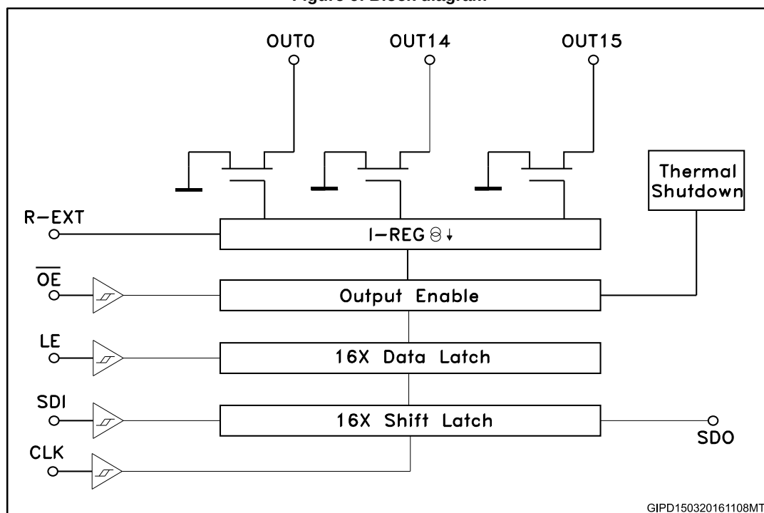
Figure 6: Block diagram
