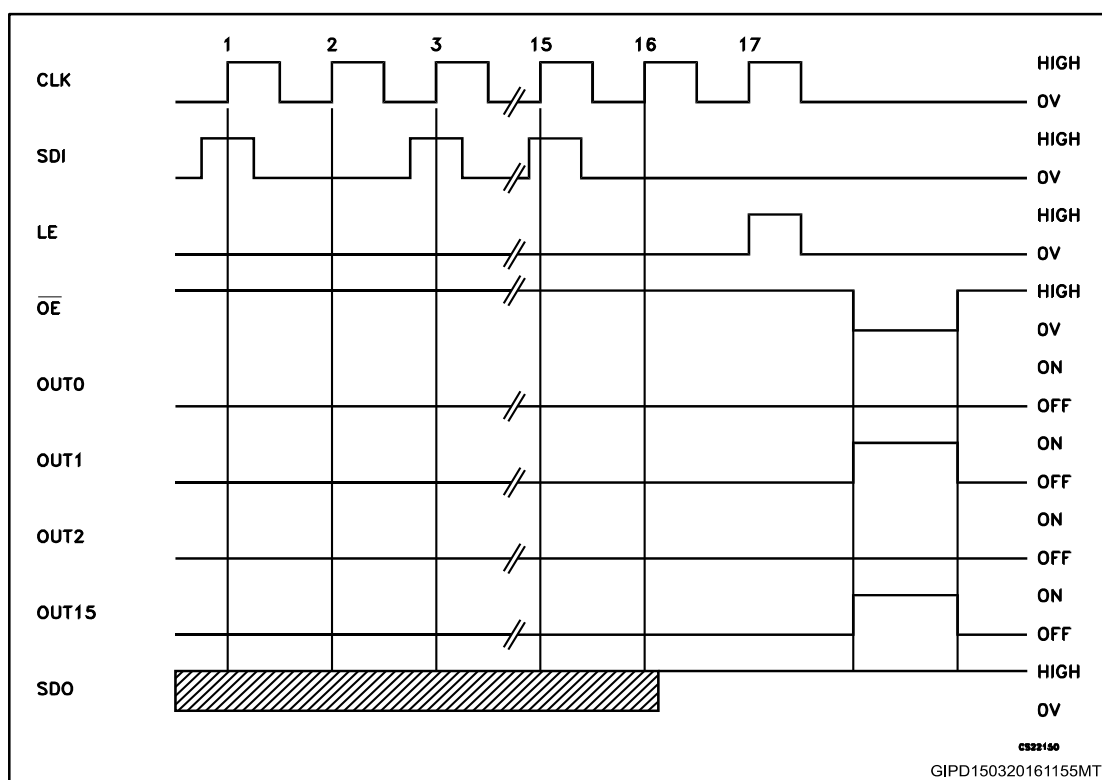
Figure 7: Timing diagram
