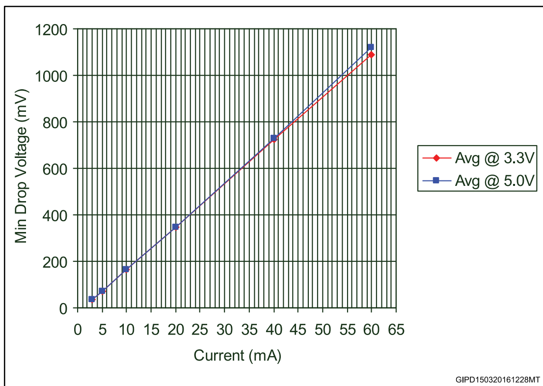
Figure 13: I SET vs drop out voltage (V drop )
