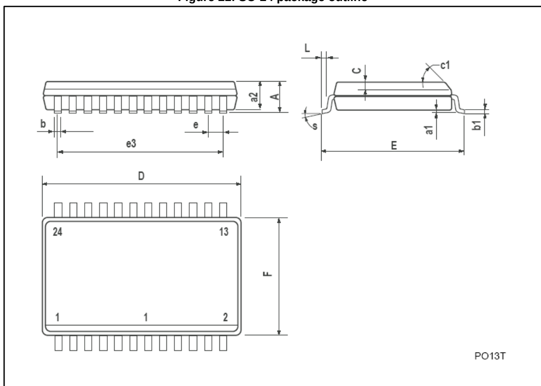
Figure 21: SO-24 package outline
