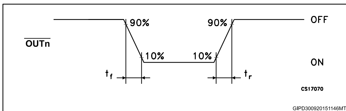
Figure 10: Outputs
