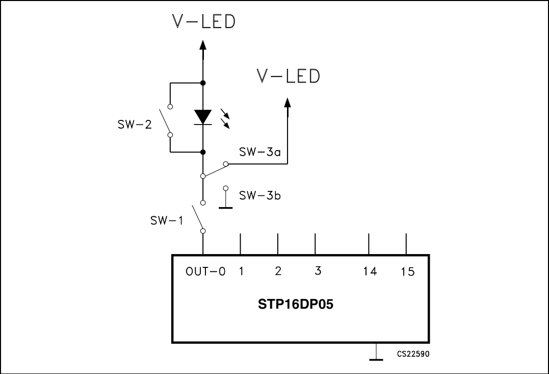
Figure 19. Detection circuit
