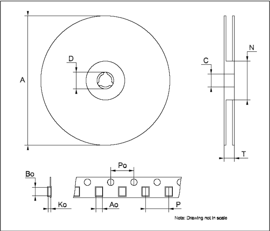
Figure 25. Reel dimensions
