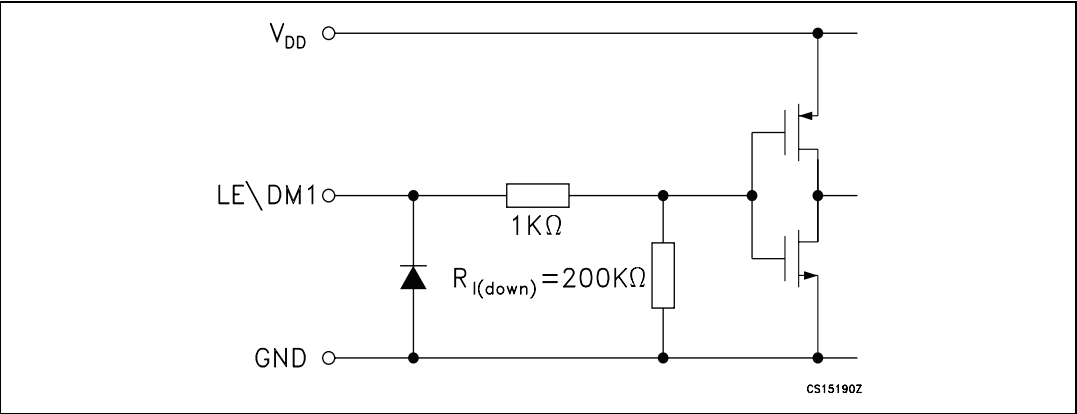
Figure 3. \text{LE}\backslash\text{DM1} terminal
