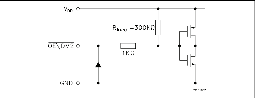
Figure 2. \overline{\text{OE}}\backslash\text{DM2} terminal
