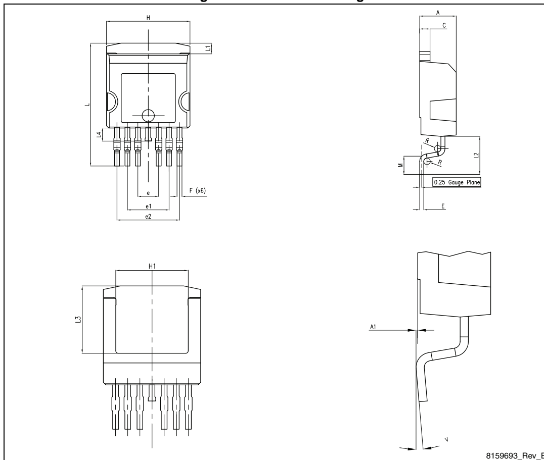
Figure 26. H 2 PAK-6 drawing
