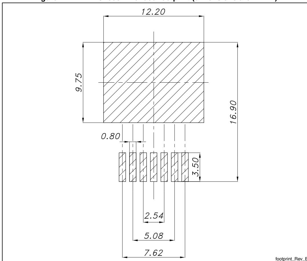
Figure 27. H 2 PAK-6 recommended footprint (dimensions are in mm)
