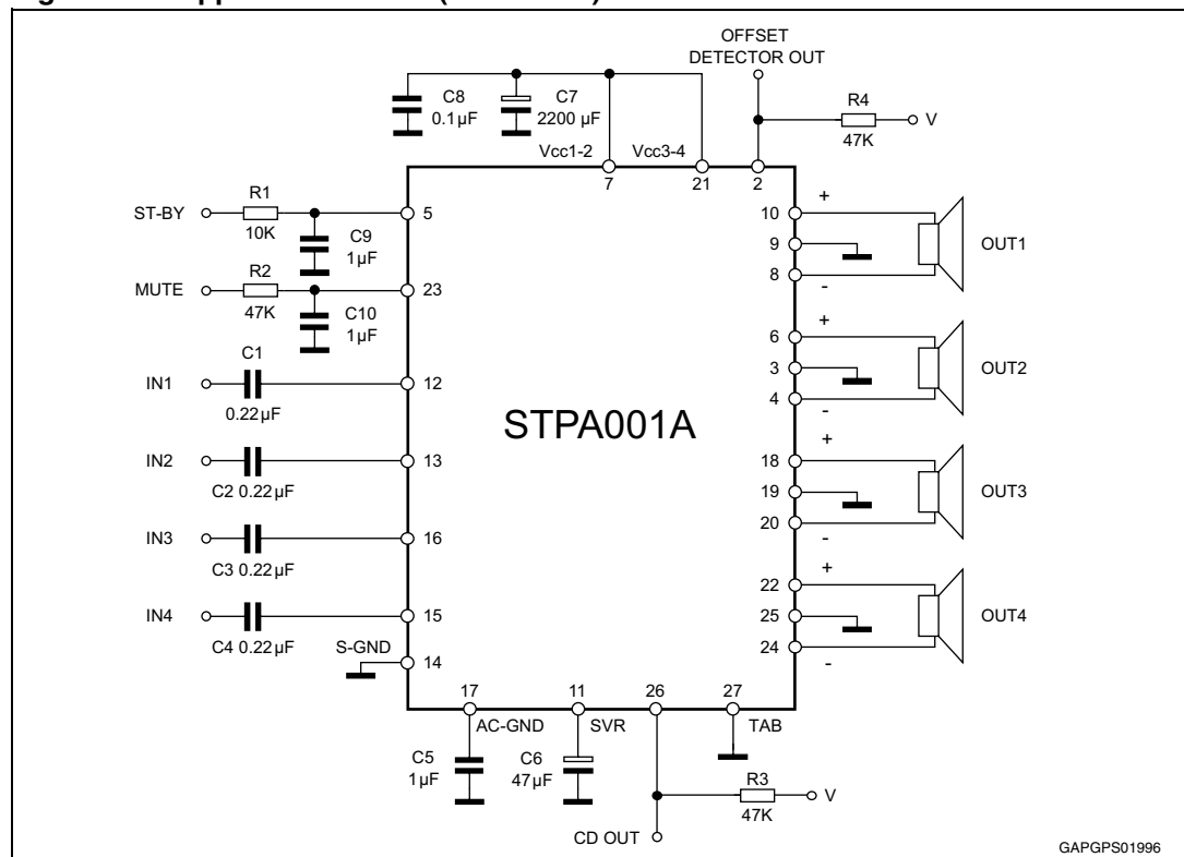
Figure 3. Application circuit (STPA001A)
