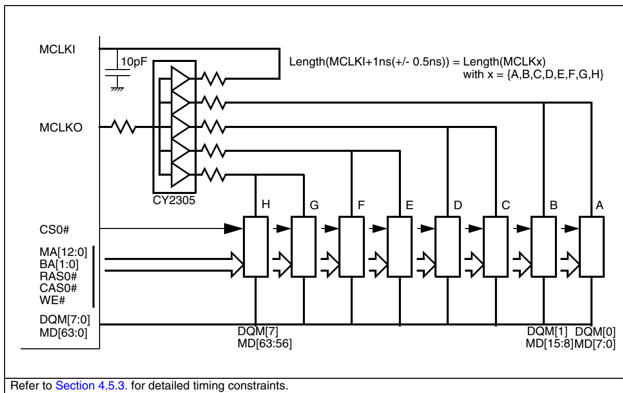
Figure 6-6. One Memory Banks with 8 Chips (8-bit)
