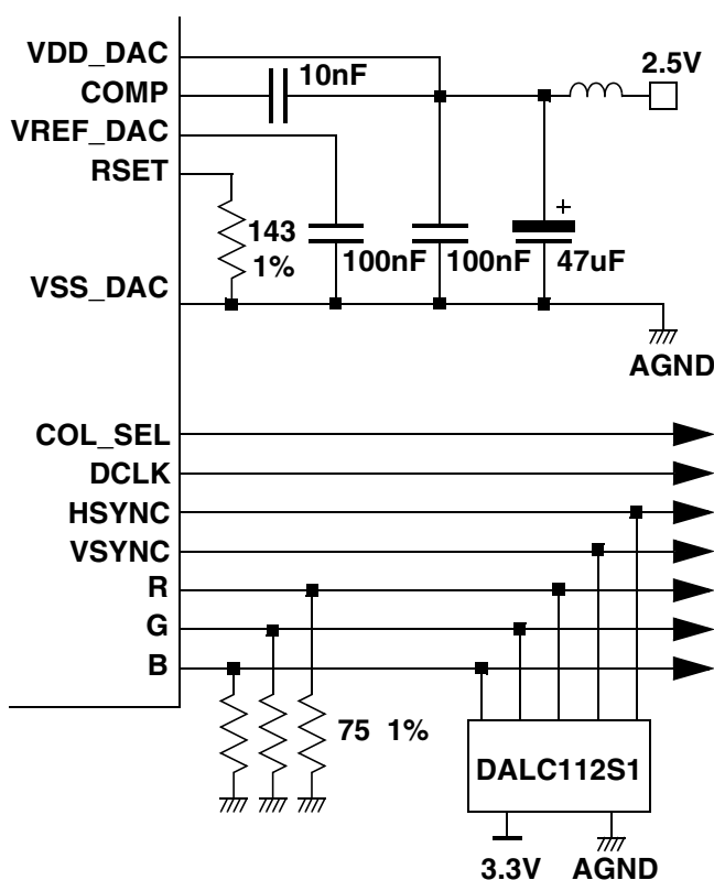
Figure 6-15. Typical VGA implementation
