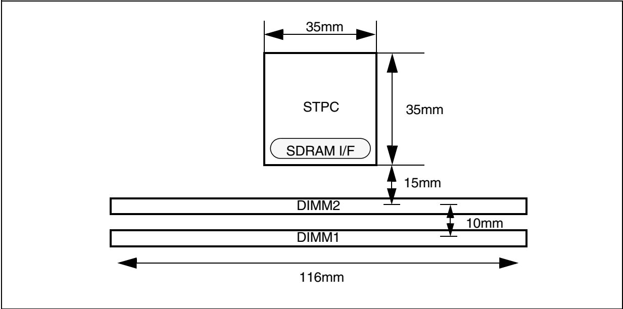
Figure 6-22. DIMM placement
