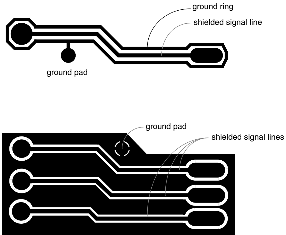
Figure 6-20. Shielding signals
