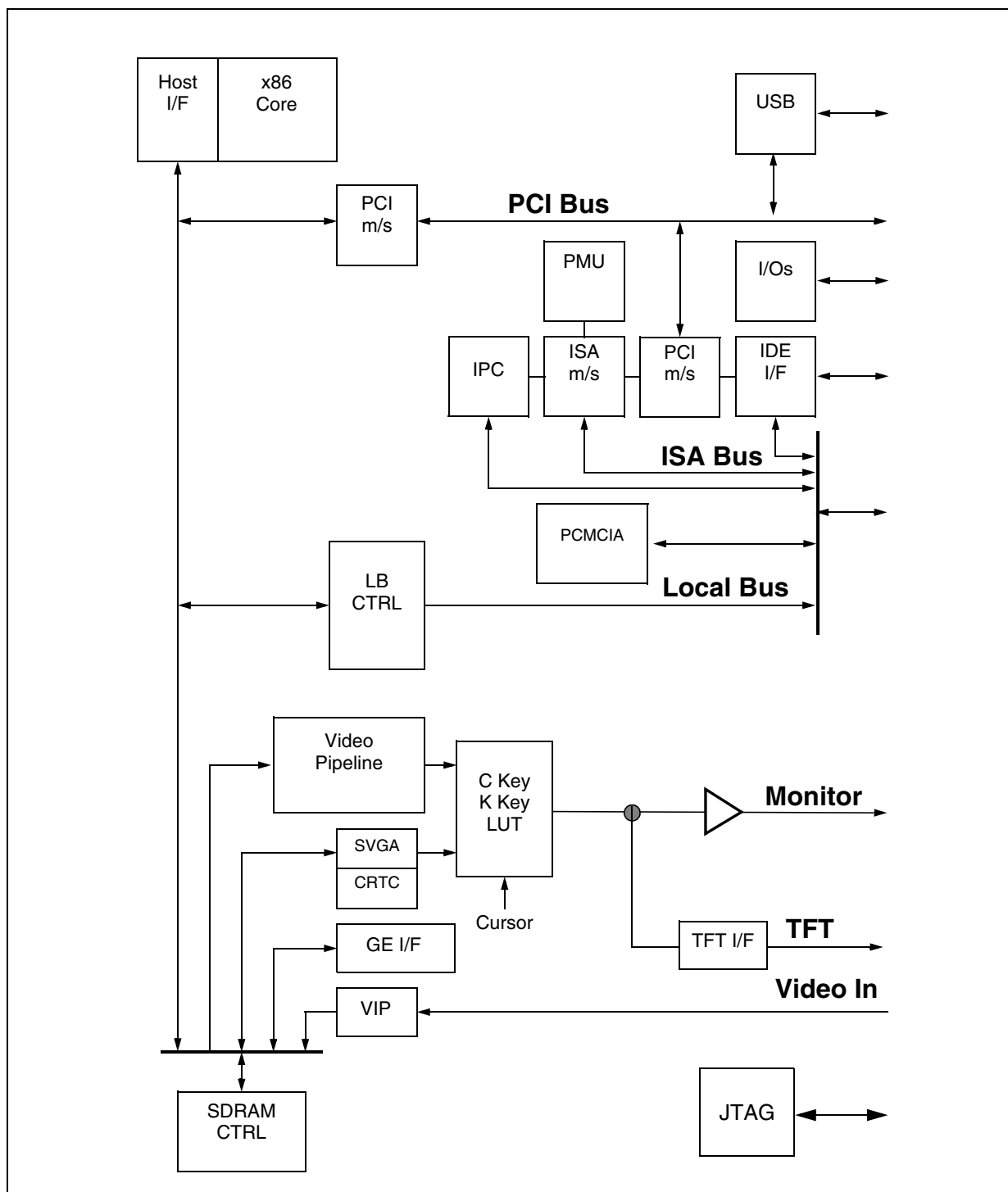
Figure 1-1. Functional description.
