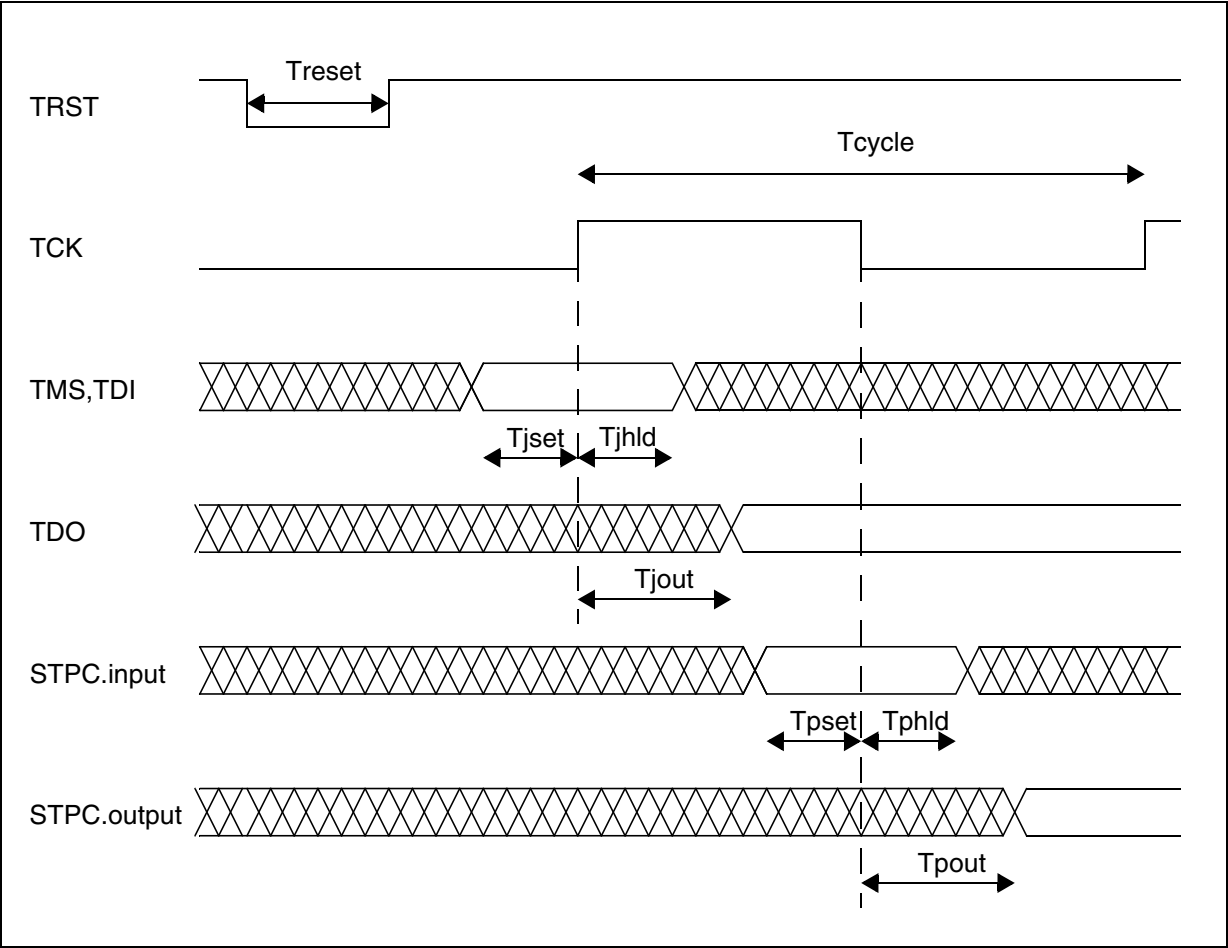
Figure 4-15. JTAG timing diagram
