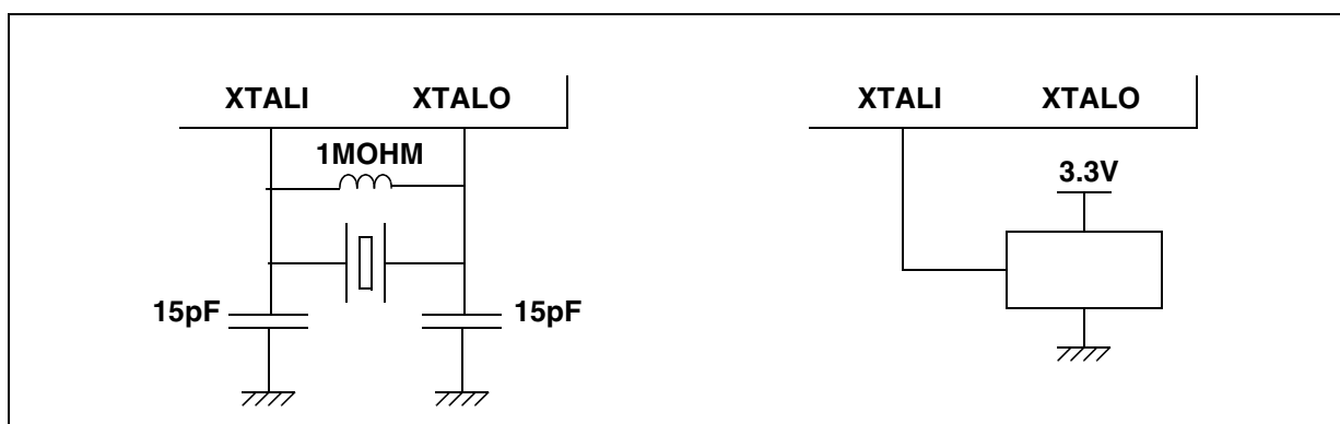
Figure 6-4. 14.31818 MHz stage
