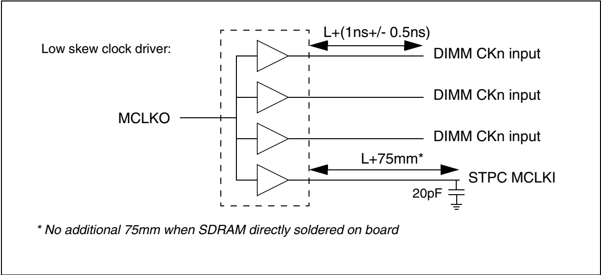
Figure 6-23. Clock Routing
