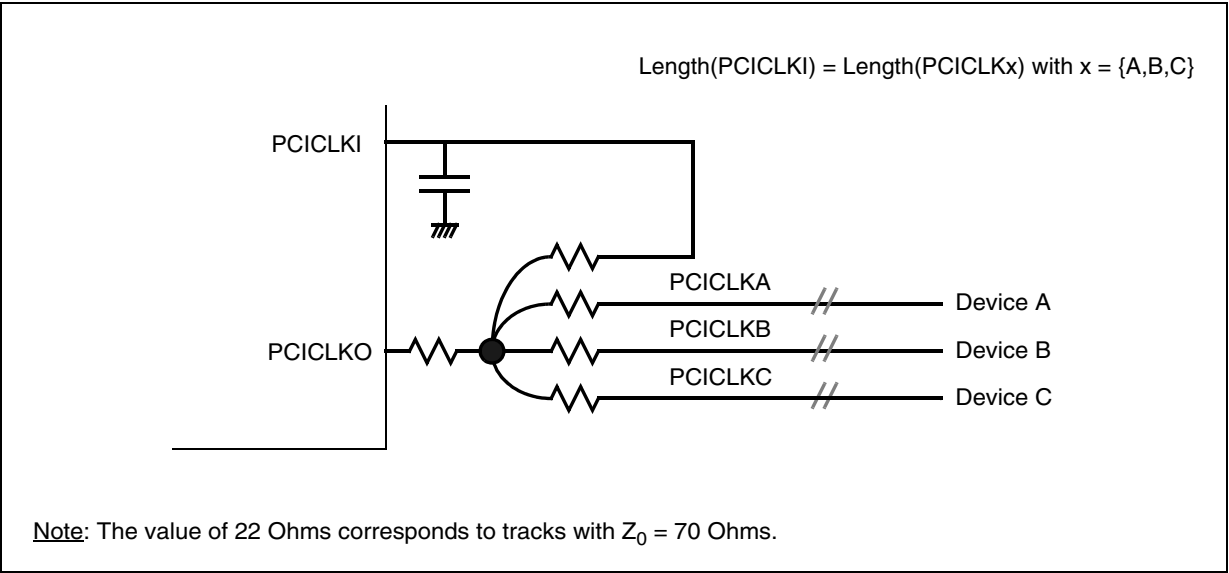
Figure 6-30. Clocks relationships
