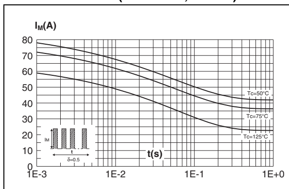
Figure 5. Non repetitive surge peak forward current versus overload duration - maximum values, per diode (TO-220AB, D 2 PAK)
