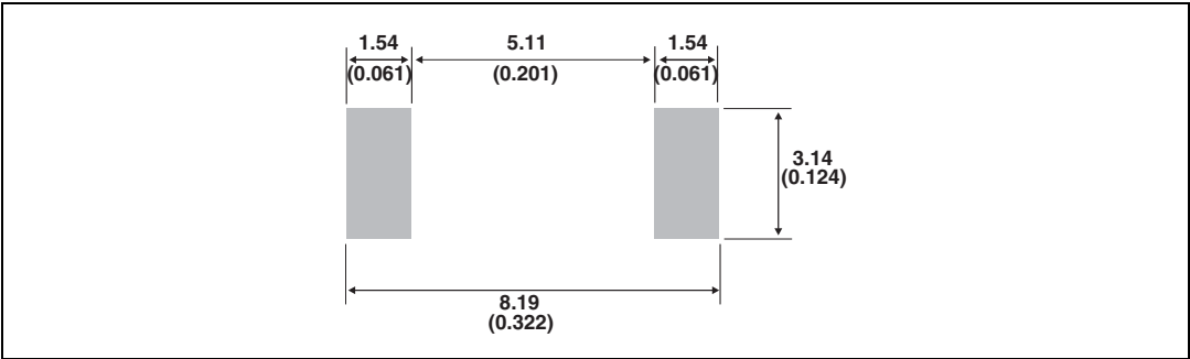
Figure 24. SMC footprint, dimensions in mm (inches)
