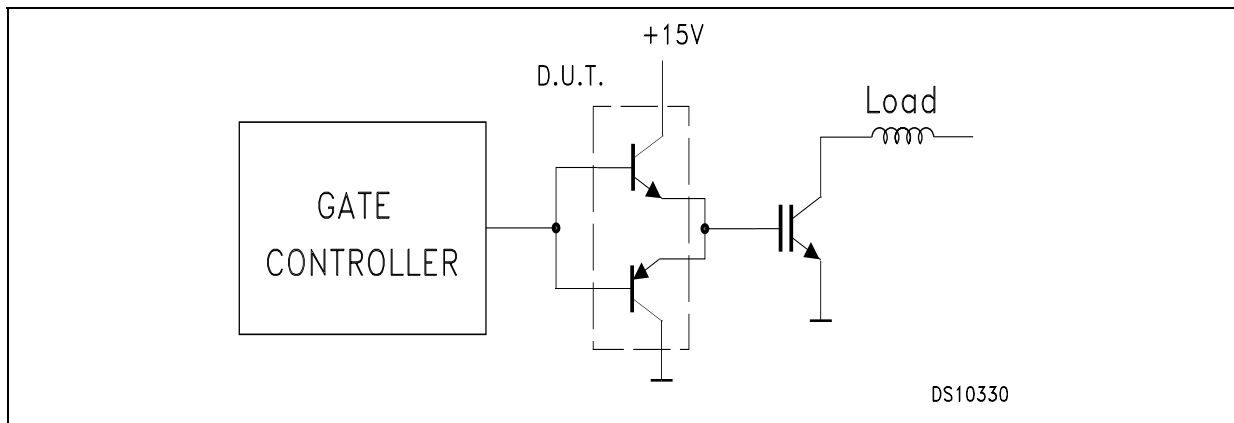
Figure 3: Typical Application
