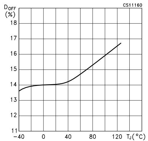
Figure 10 : Duty Cycle Shut Down vs Temperature
