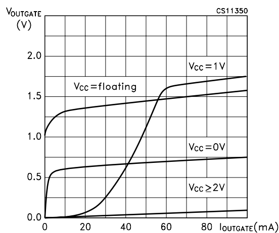
Figure 3 : V_{OUTGATE} vs Characteristics
