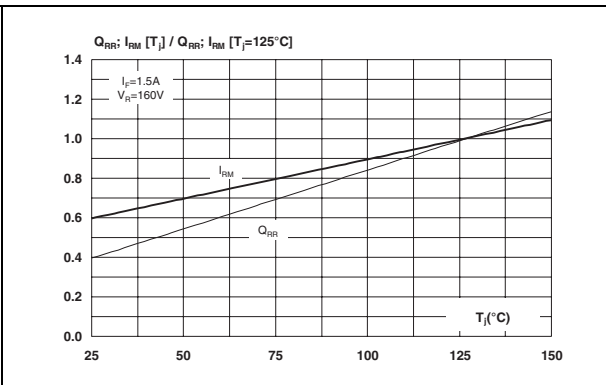
Figure 12. Dynamic parameters versus junction temperature
