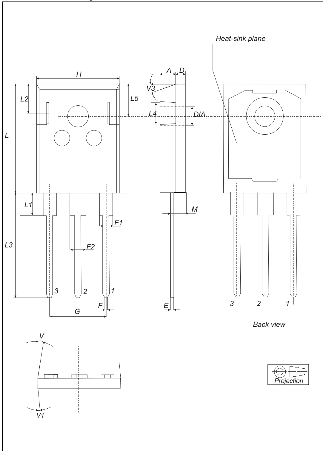
Figure 16. TO-247 LL dimension definitions
