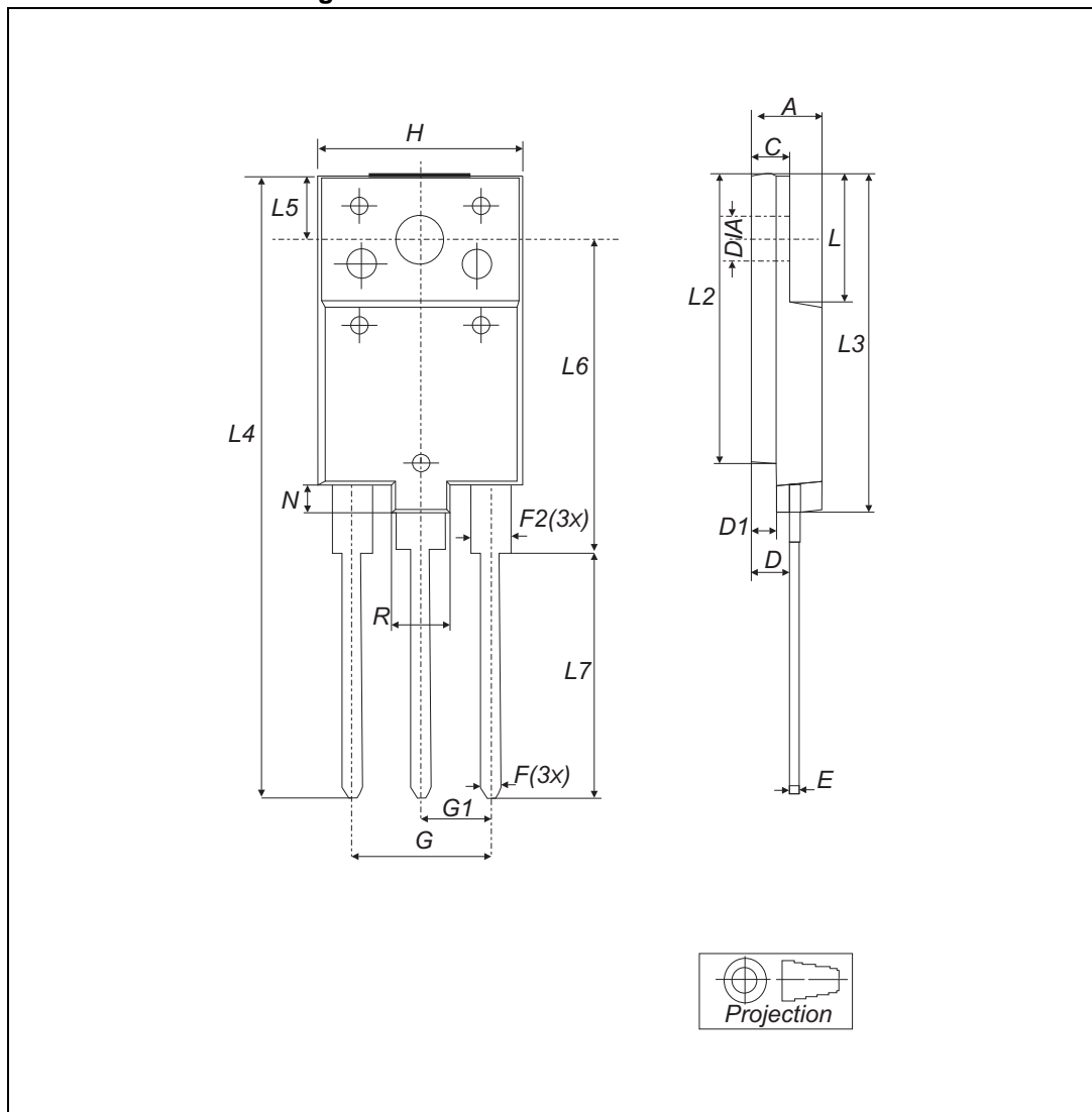
Figure 15. TO-3PF dimension definitions
