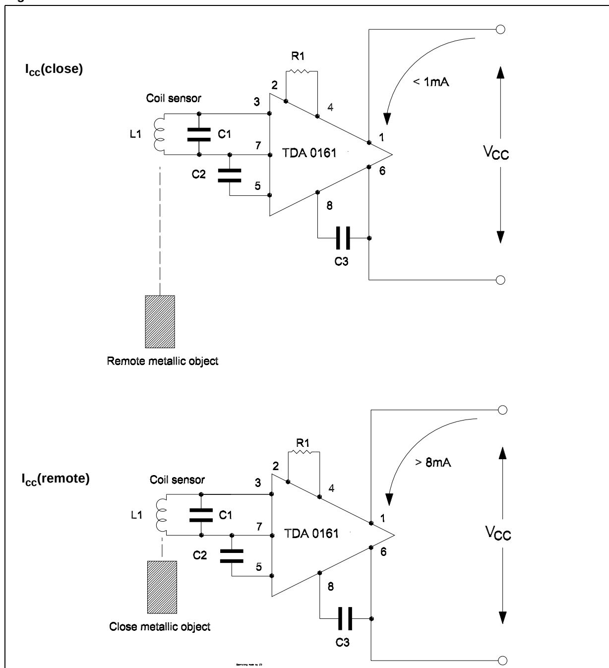
Figure 2. Electrical Scheme
