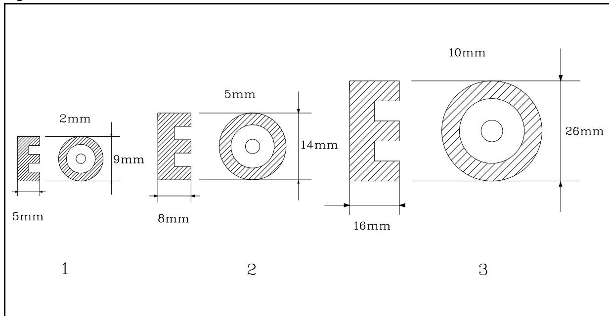
Figure 4. Detection distance
