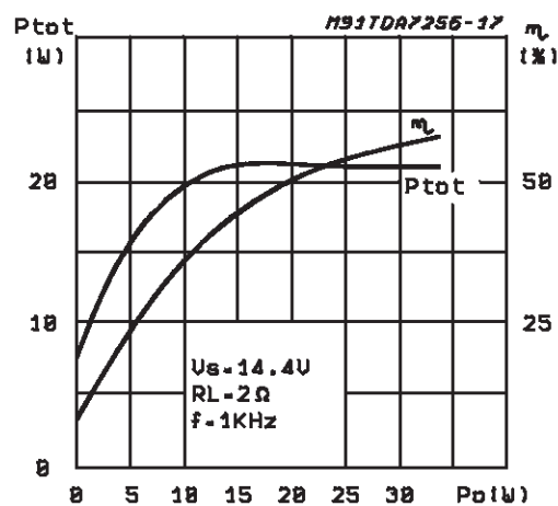
Figure 16: Power Dissipation &amp; Efficiency vs. Output Power
