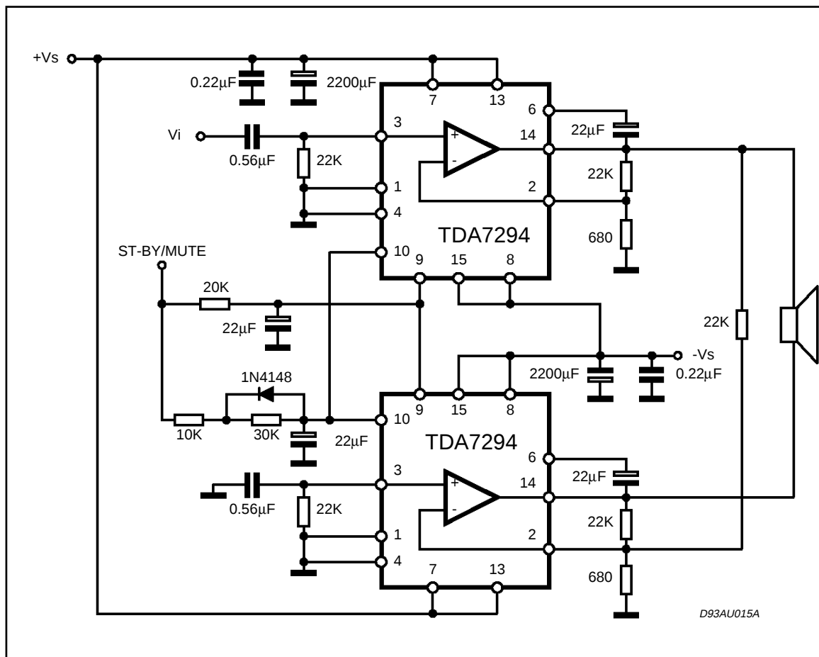
Figure 18: Bridge Application Circuit
