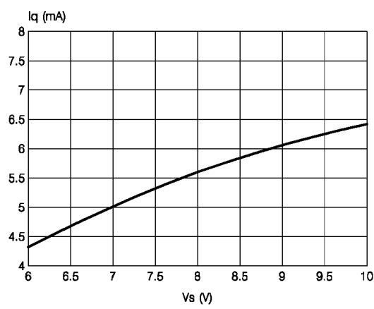
Figure 11. Quiescen Current vs. Supply Voltage
