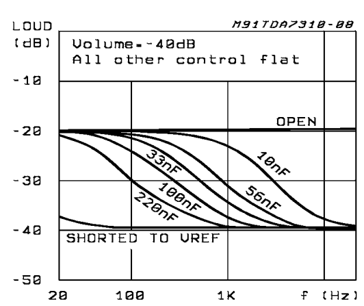
Figure 14. Loudness vs. External Capacitors
