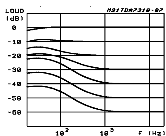
Figure 13. Loudness vs. Frequency (C LOAD = 100nF) vs. Volume
