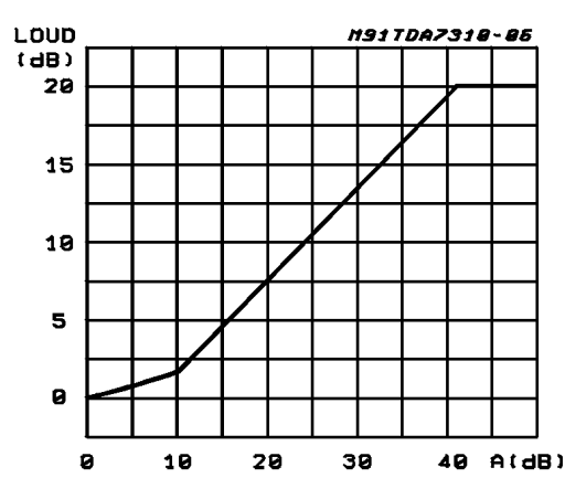
Figure 12. Loudness vs. Volume Attenuation
