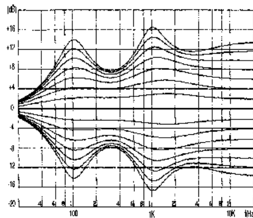
Figure 12. Typical tone response
