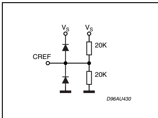
Figure 20. Pins 1, 2, 3, 4, 5, 6, 7, 28
