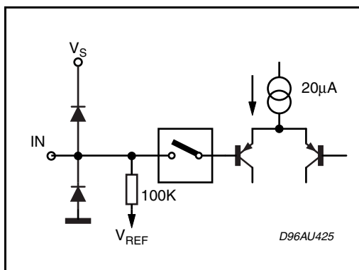
Figure 22. Pins 11, 16
