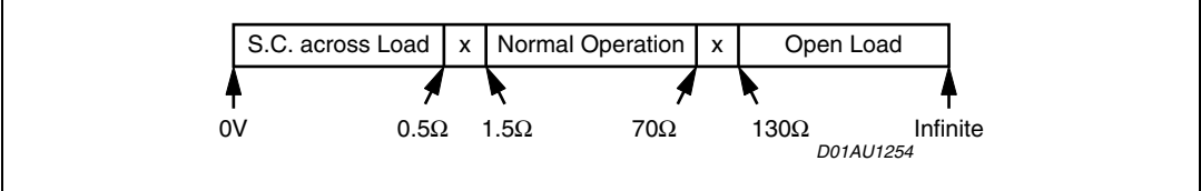
Figure 33. Load detection thresholds - high gain setting
