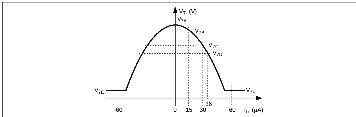
Figure 2 : Parabola Characteristics
