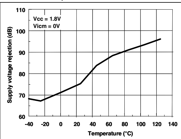
Figure 8. Supply voltage rejection vs. temperature at Vcc = 1.8 V
