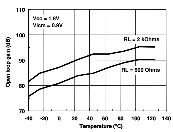
Figure 12. Open loop gain vs. temperature at Vcc = 1.8 V
