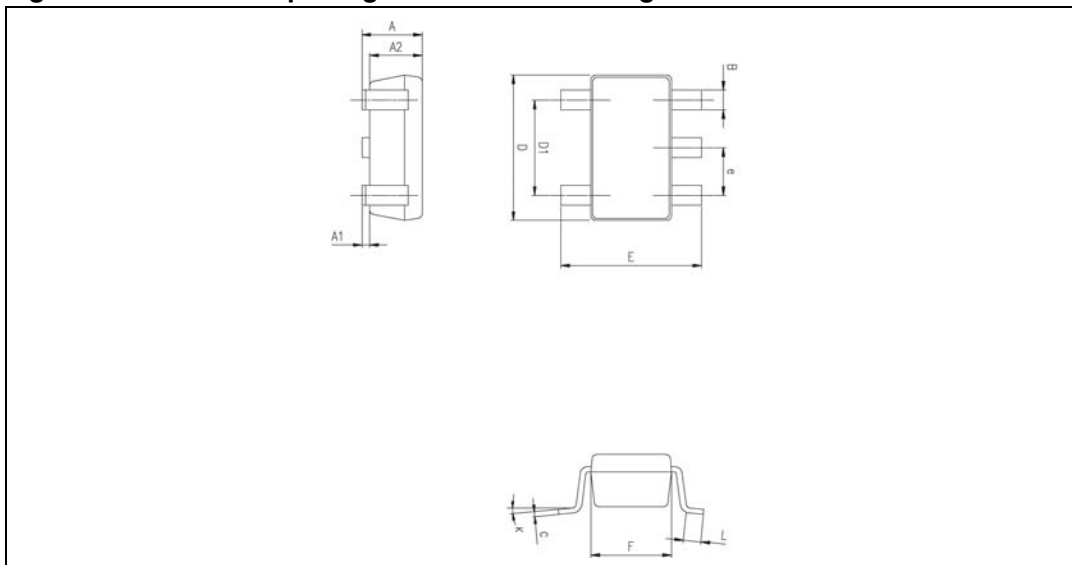
Figure 54. SOT23-5L package mechanical drawing
