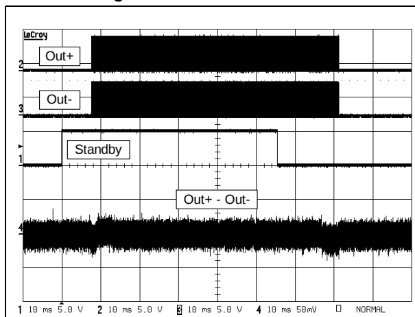
Figure 34. Startup and shutdown phase V_{CC} = 5V , G = 6dB , C_{in} = 1\mu F , inputs grounded
