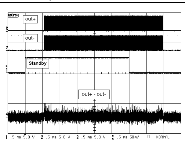
Figure 43. Startup and shutdown phase V_{CC}=5V , G=6dB , C_{in}=1\mu F , inputs grounded
