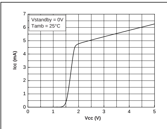
Fig. 72 : Current Consumption vs Power Supply Voltage
