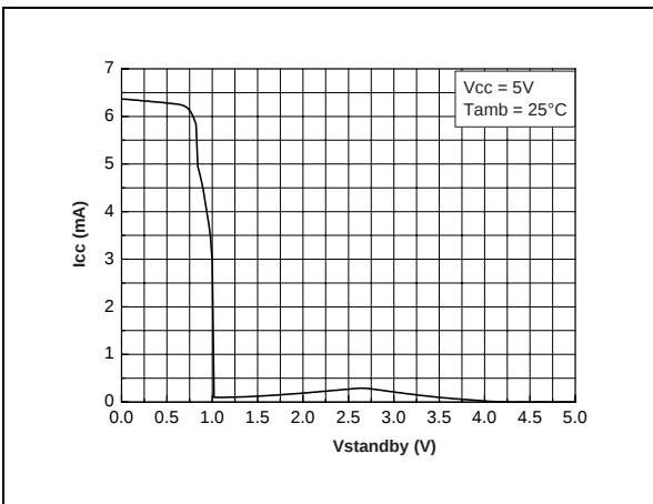
Fig. 74 : Current Consumption vs Standby Voltage @ V_{CC} = 5V
