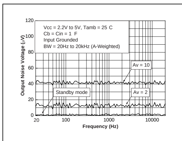
Fig. 102 : V_{out1}+V_{out2} A-weighted Noise Floor
