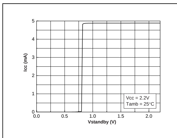
Fig. 98 : Current Consumption vs Standby Voltage @ V_{CC} = 2.2V
