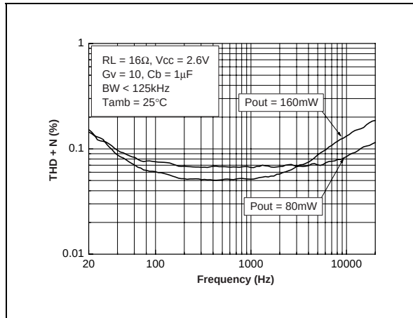
Fig. 85 : THD + N vs Frequency
