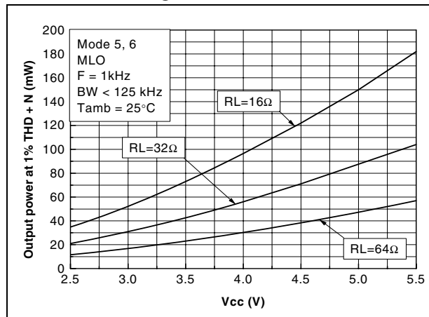
Figure 44. Output power vs. power supply voltage
