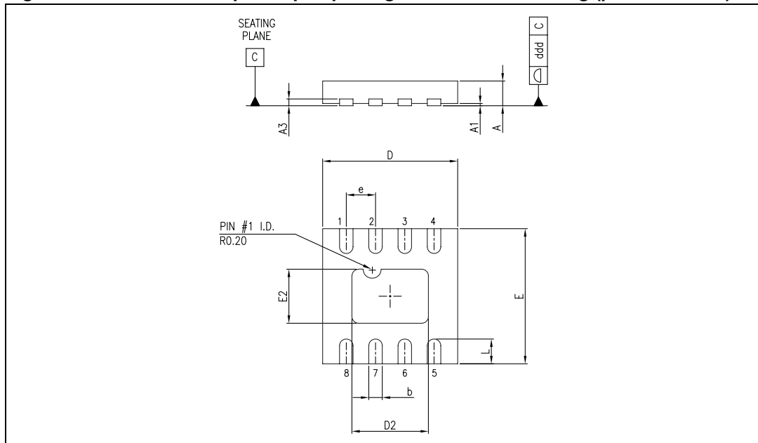
Figure 71. DFN8 3 x 3 exposed pad package mechanical drawing (pitch 0.65 mm)
