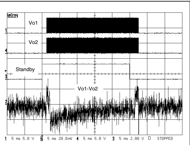
Figure 57. Startup and shutdown times V_{CC} = 5V, G = 6dB, C_{in} = 100nF (5ms/div)
