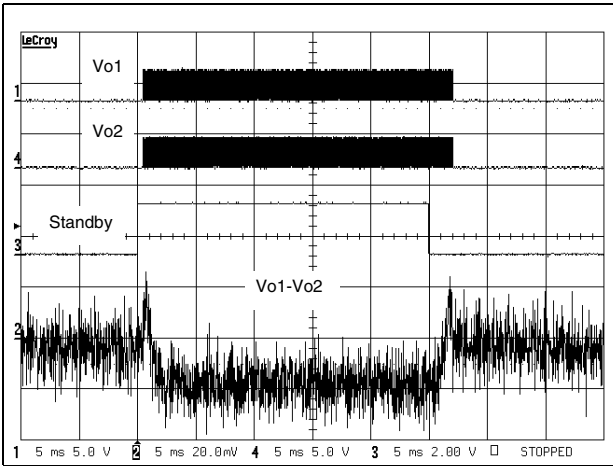
Figure 60. Startup and shutdown times V_{CC} = 3V , G = 6dB , No C_{in} (5ms/div)
