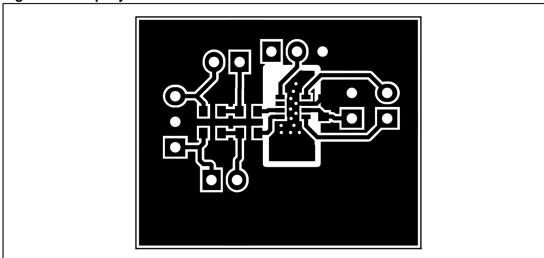
Figure 69. Top layer
