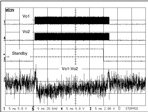
Figure 58. Startup and shutdown times V_{CC} = 3V , G = 6dB , C_{in} = 100nF (5ms/div)
