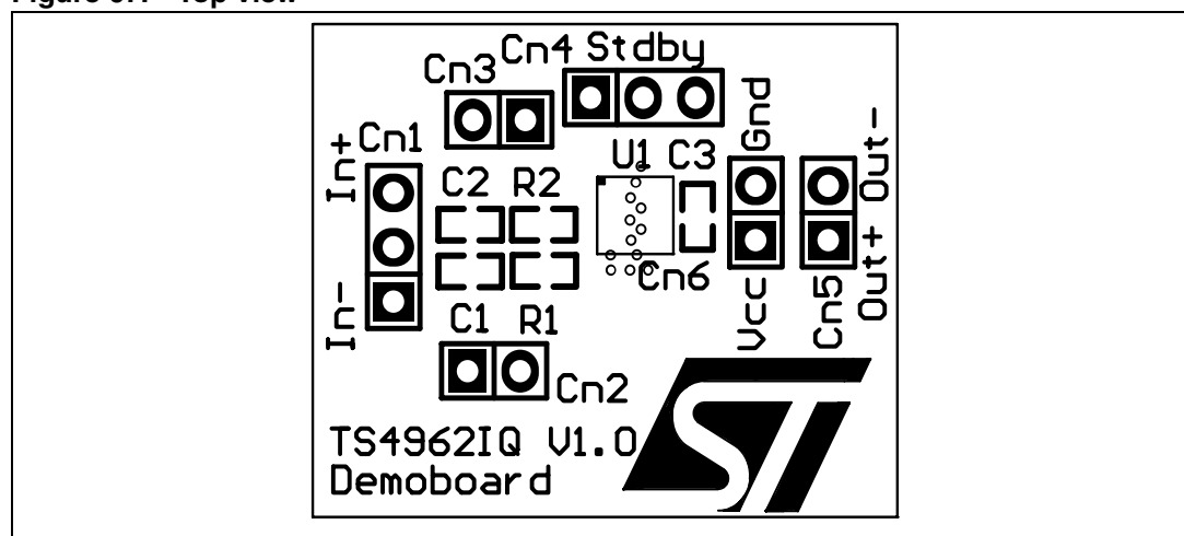
Figure 67. Top view
