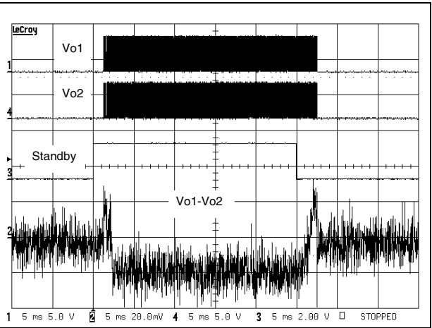
Figure 59. Startup and shutdown times V_{CC} = 5V , G = 6dB , No C_{in} (5ms/div)
