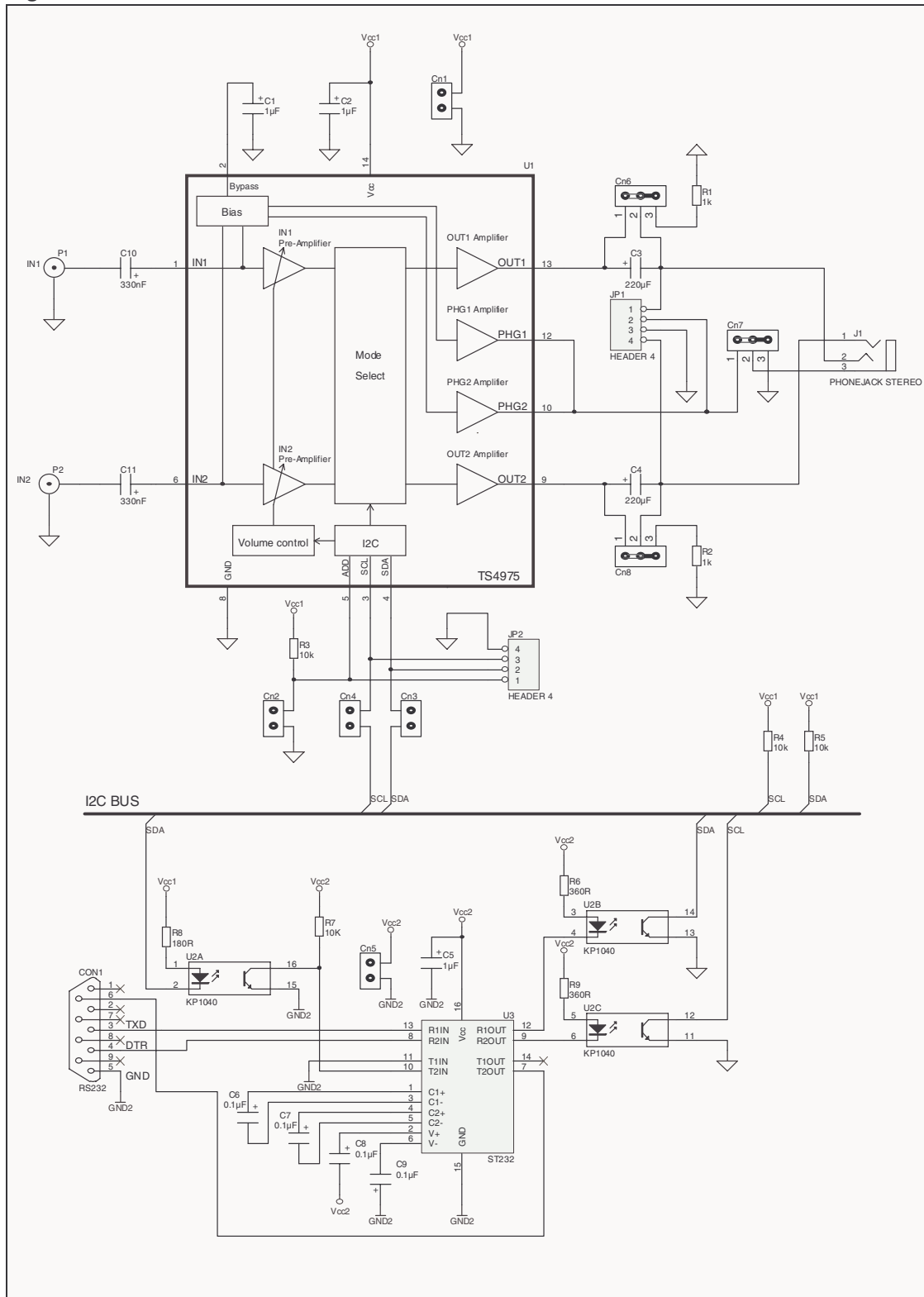
Figure 67. Demoboard schematic
