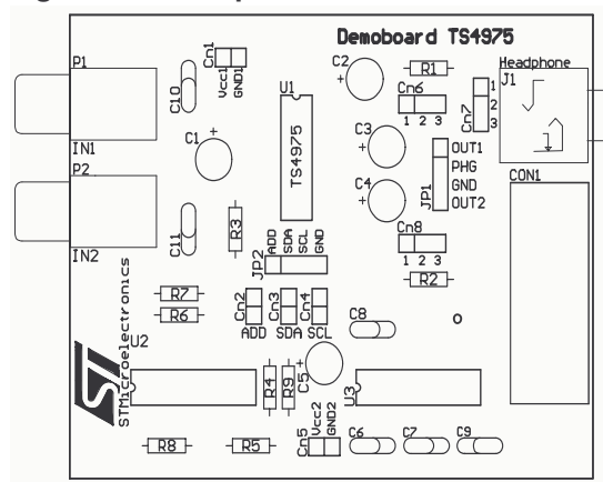
Figure 66. Component location
