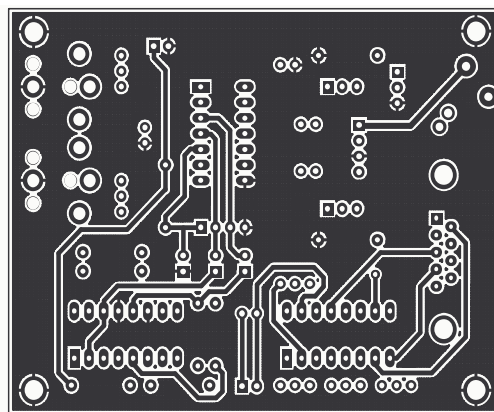
Figure 65. Top layer
