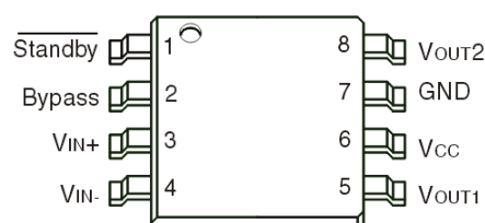
TS4990IQT - DFN8
