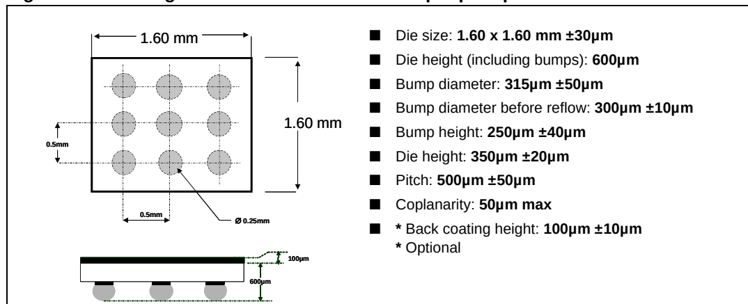
Figure 67. Package mechanical data for 9-bump flip-chip
