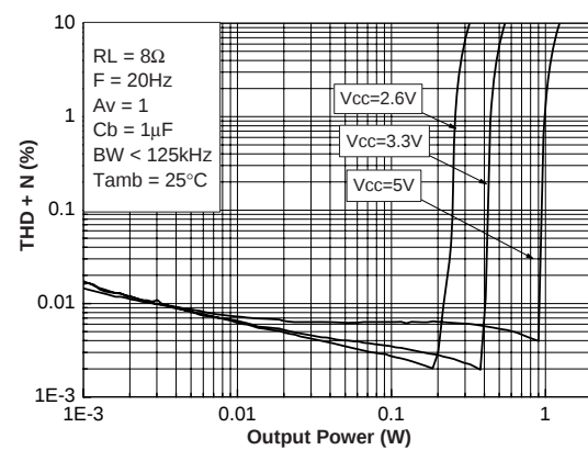
Figure 44. THD+N vs. output power
