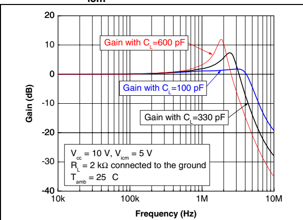
Figure 17. Frequency response for different capacitive loads at V_{CC} = 10 V, V_{icm} = 5 V and T = 25^\circ\text{C}
