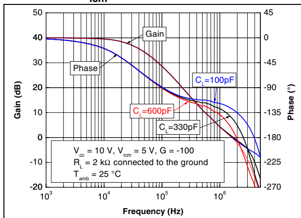
Figure 14. Voltage gain and phase for different capacitive loads at V_{CC} = 10 V, V_{icm} = 5 V and T = 25^\circ\text{C}
