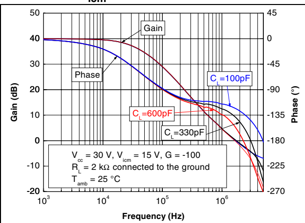
Figure 15. Voltage gain and phase for different capacitive loads at V_{CC} = 30 V, V_{icm} = 15 V and T = 25^\circ\text{C}
