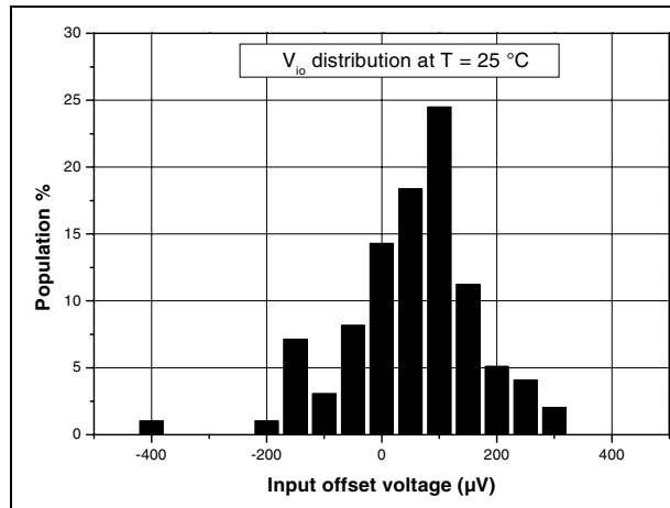
Figure 2. V_{io} distribution at V_{cc} = \pm 15 V and T = 25^\circ\text{C}
