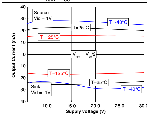
Figure 12. Output current vs. supply voltage at V_{icm}=V_{cc}/2
