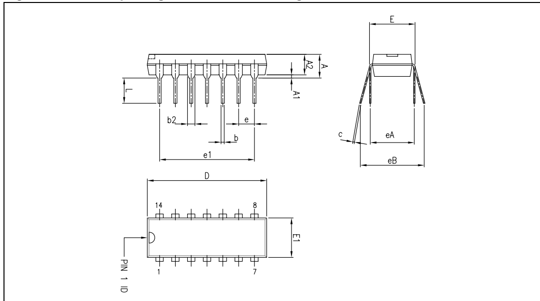
Figure 16. DIP14 package mechanical drawing
