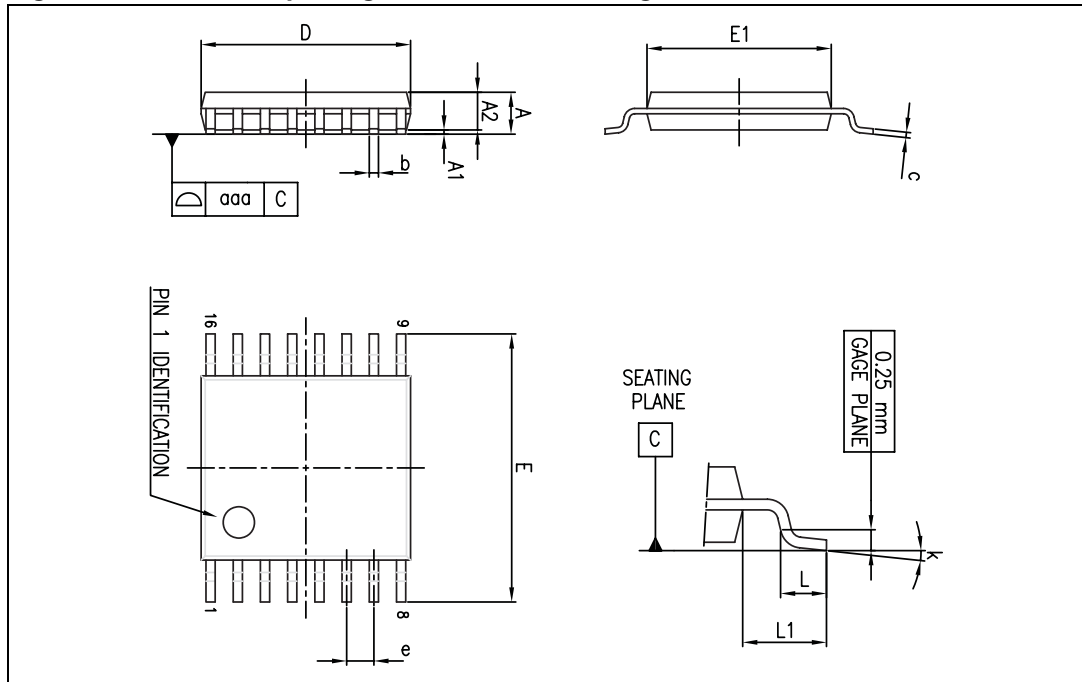
Figure 22. TSSOP16 package mechanical drawing
