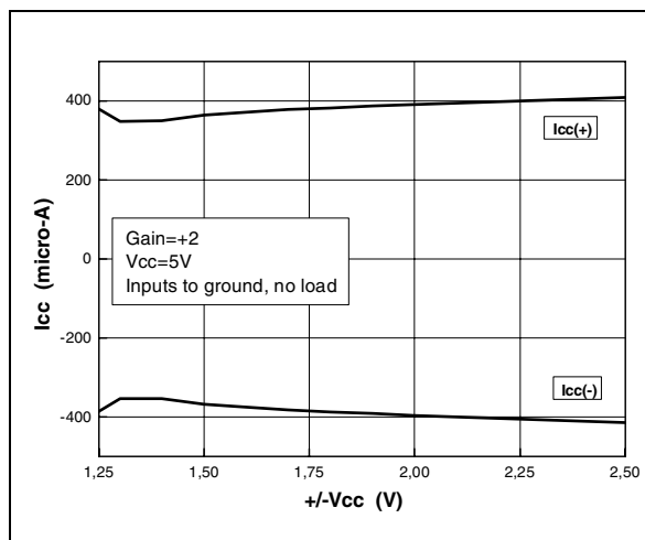
Figure 11: Isource
