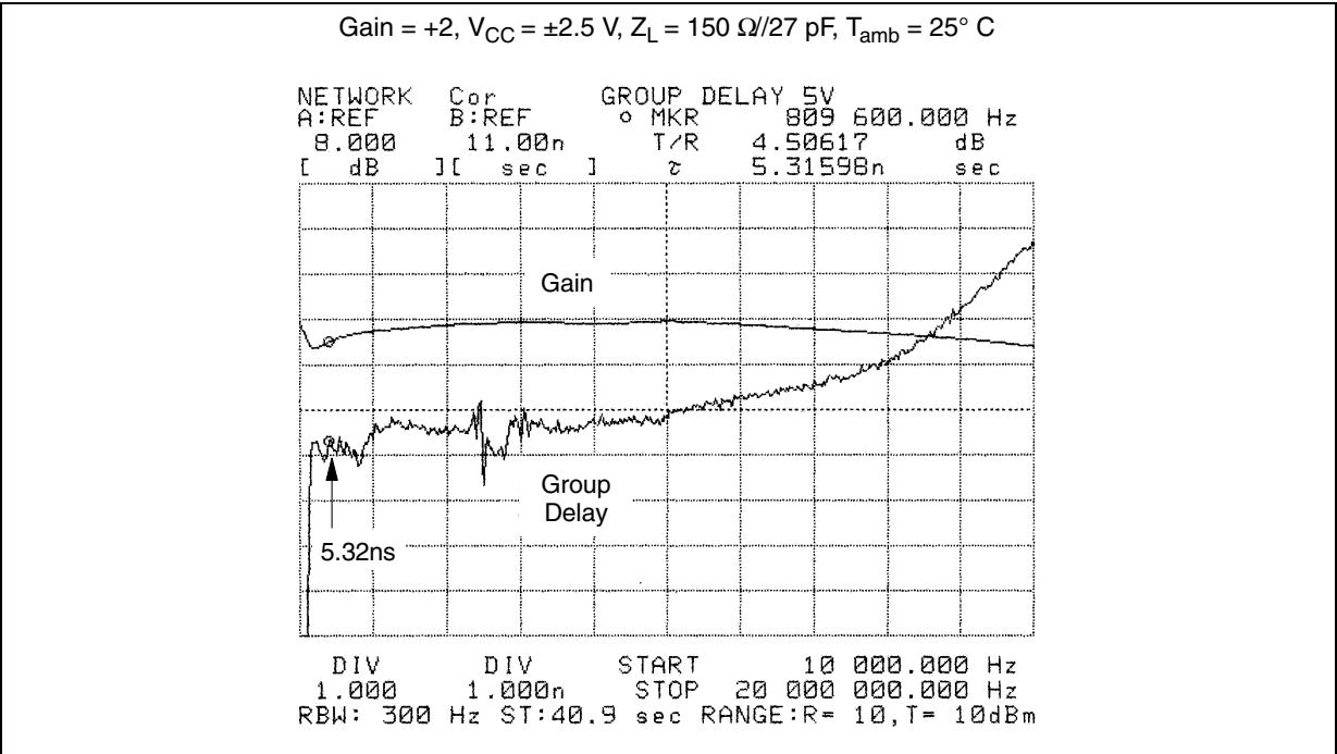
Figure 15. Group delay
