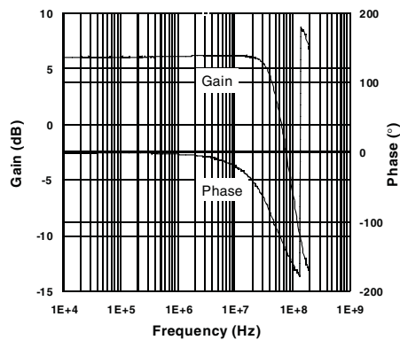
Figure 3. Closed loop gain and phase vs. frequency
