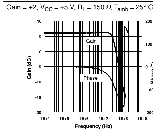
Figure 16. Closed loop gain and phase vs. frequency
