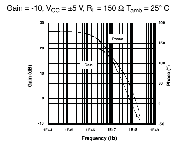
Figure 18. Closed loop gain and phase vs. frequency
