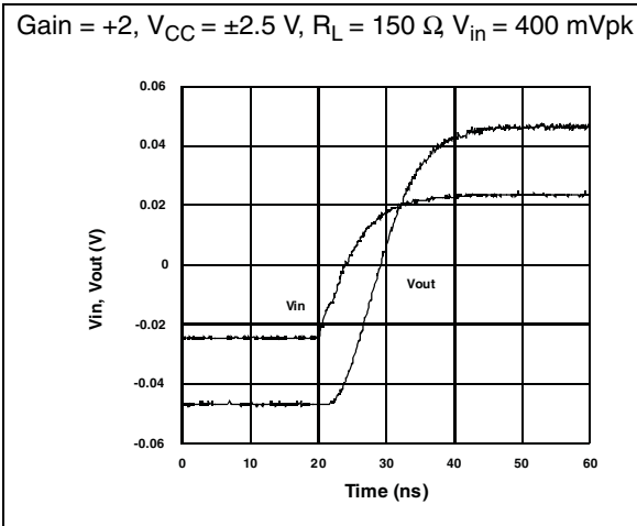
Figure 7. Small signal measurement - rise time
