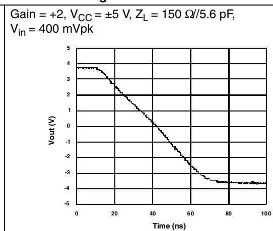
Figure 21. Large signal measurement - negative slew rate
