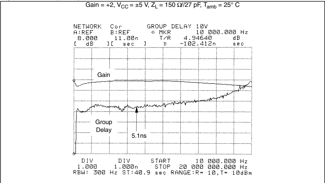
Figure 30. Group delay
