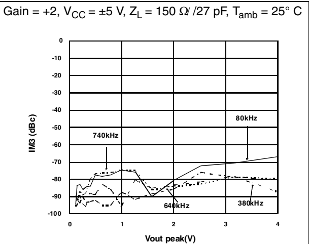
Figure 29. Third order intermodulation (1)
