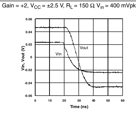
Figure 8. Small signal measurement - fall time
