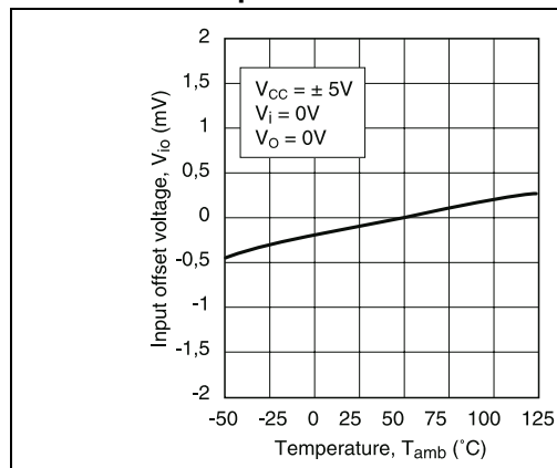
Figure 7. Input offset voltage drift versus temperature
