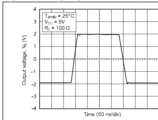
Figure 5. Large signal follower response
