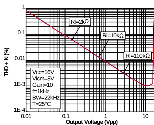
Figure 27: THD + N vs. output voltage
