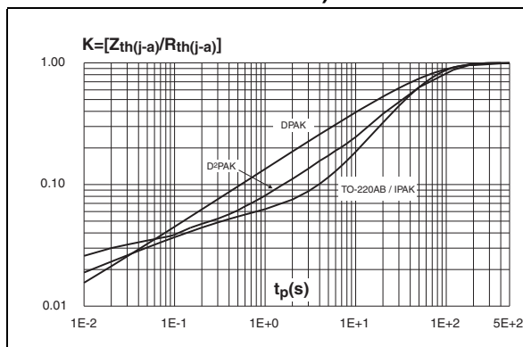
Figure 5. Relative variation of thermal impedance junction to ambient versus pulse duration (recommended pad layout, FR4 PC board for DPAK)
