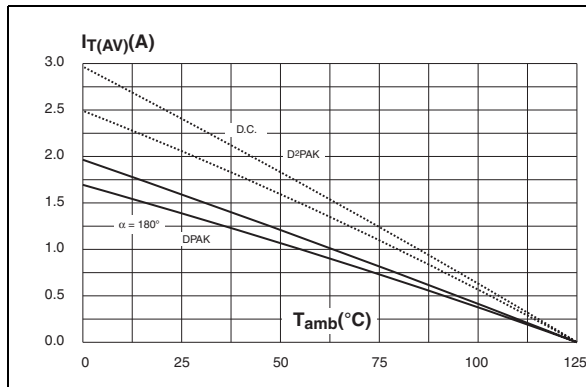
Figure 3. Average and D.C. on-state current versus ambient temperature (device mounted on FR4 with recommended pad layout) (DPAK)
