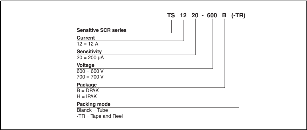
Figure 16. TS12 series
