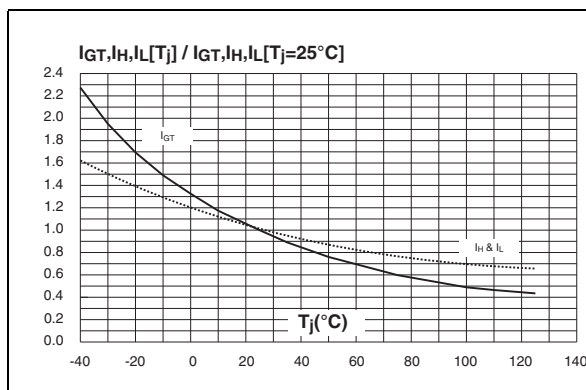
Figure 7. Relative variation of gate trigger current and holding current versus junction temperature for TN12 and TYNx12 series
