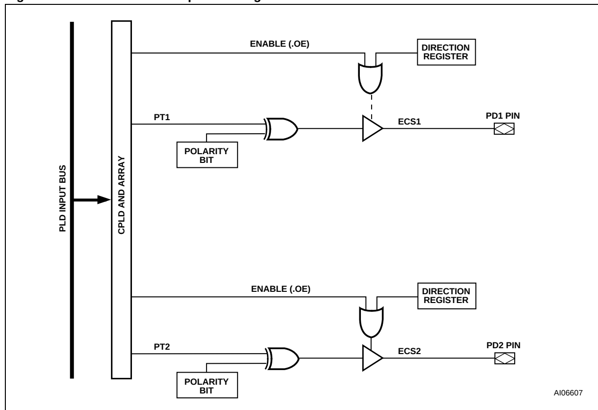
Figure 64. Port D External Chip Select Signals
