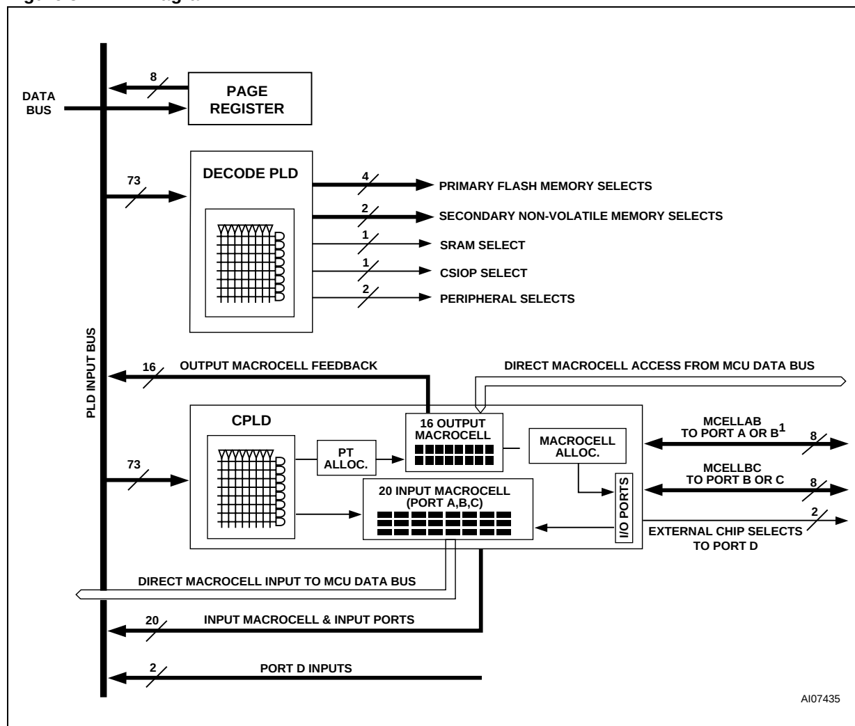
Figure 54. PLD Diagram
