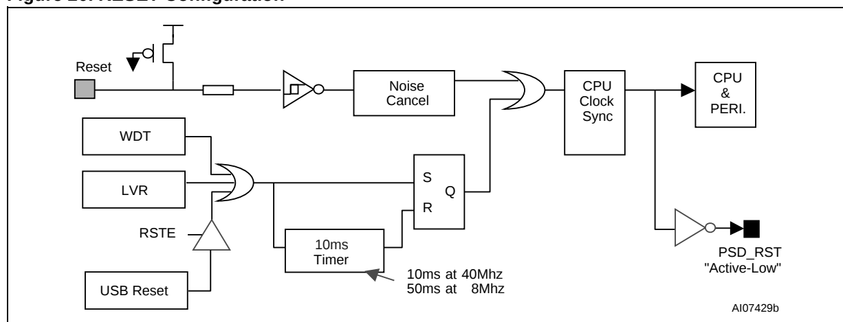
Figure 20. \overline{\text{RESET}} Configuration
