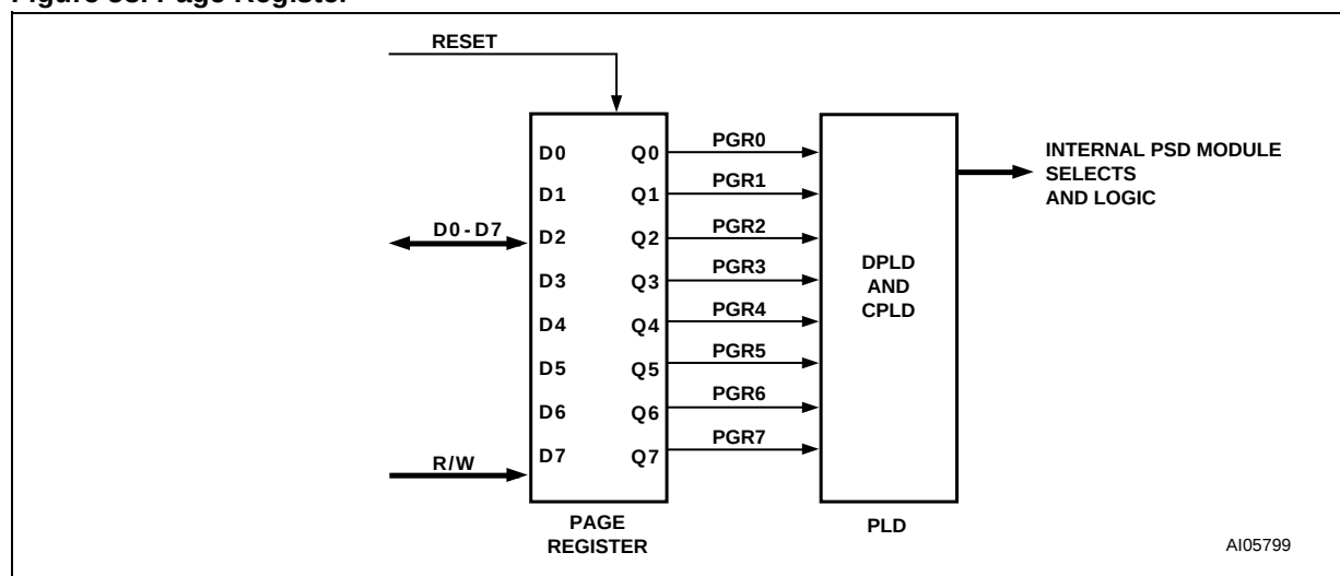
Figure 53. Page Register
