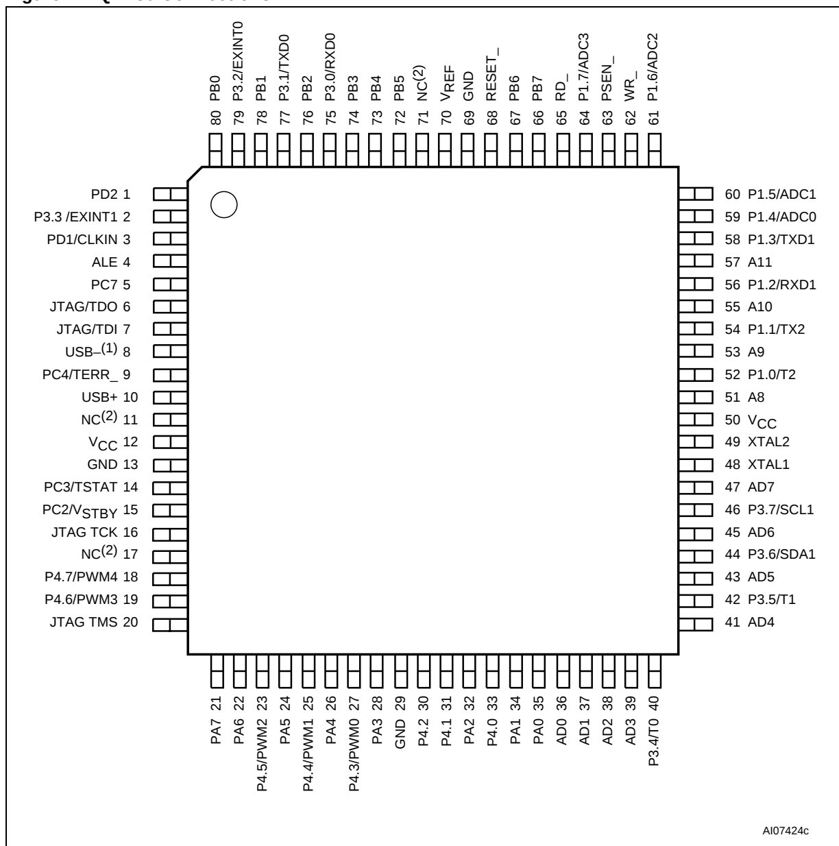
Figure 4. TQFP80 Connections
