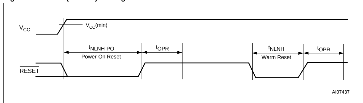
Figure 81. Reset ( \overline{\text{RESET}} ) Timing
