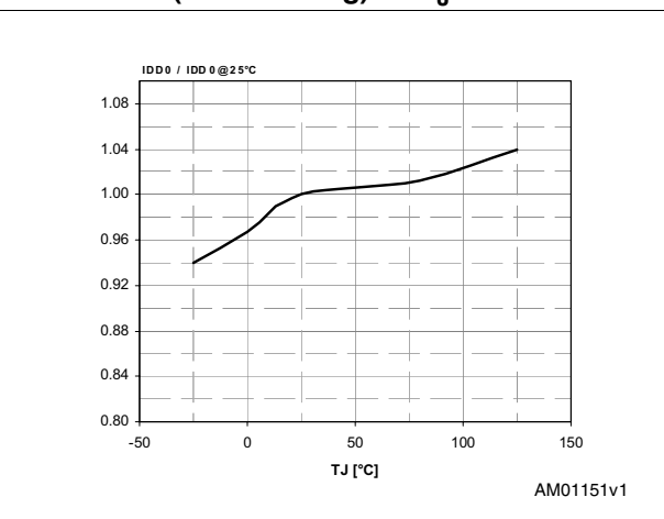
Figure 11. Operating supply current (no switching) vs T_J
