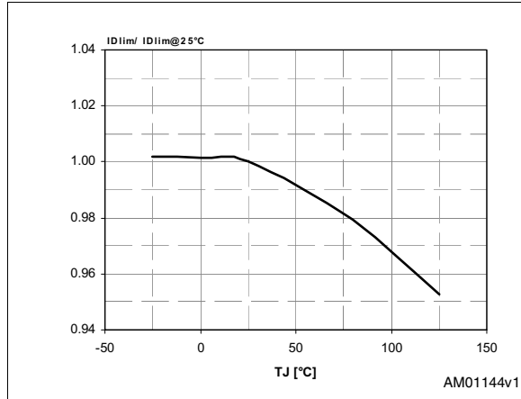
Figure 4. I_{Dlim} vs T_J
