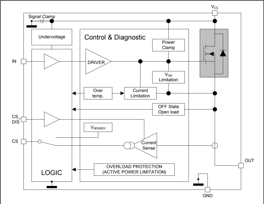
Figure 1. Block diagram
