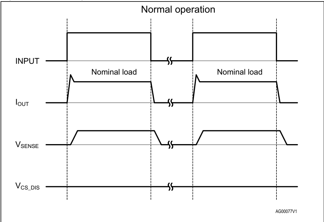
Figure 11. Normal operation
