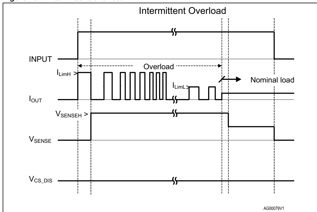
Figure 13. Intermittent overload
