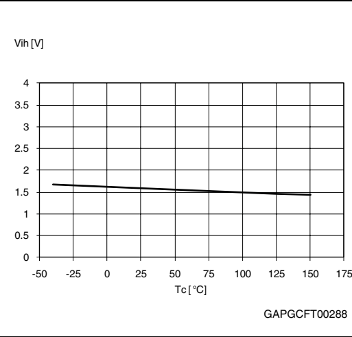
Figure 21. High-level input voltage
