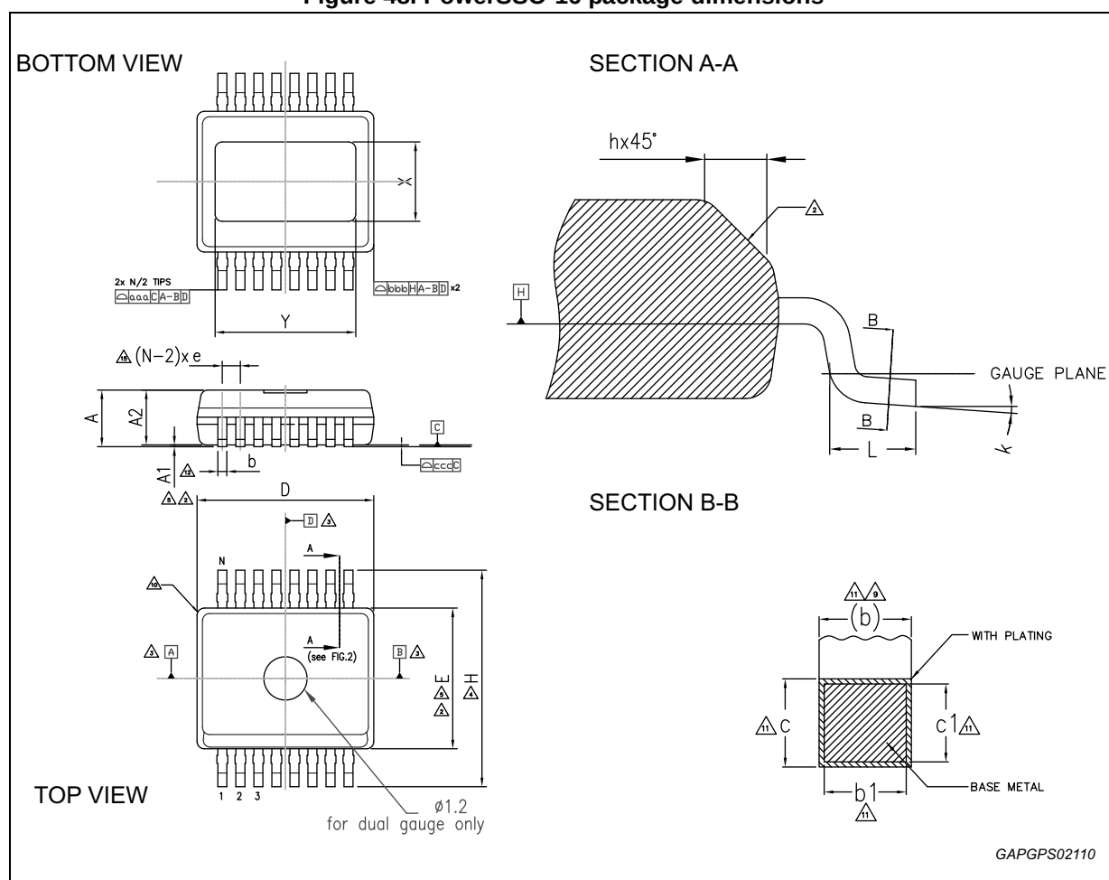
Figure 48. PowerSSO-16 package dimensions
