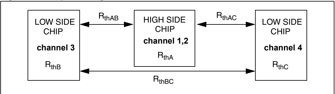
Figure 48. Chipset configuration
