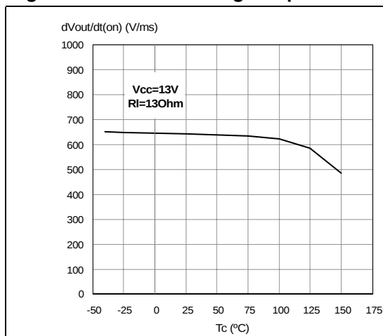
Figure 14. Turn-on voltage slope
