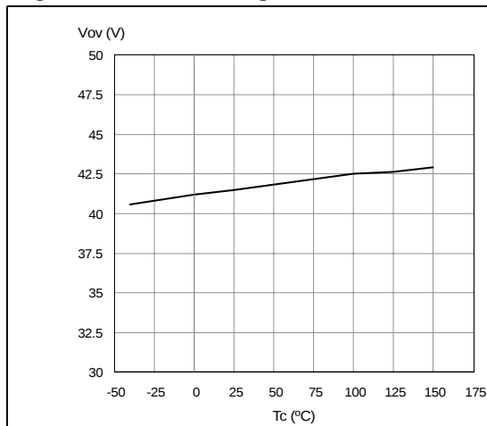
Figure 12. Overvoltage shutdown
