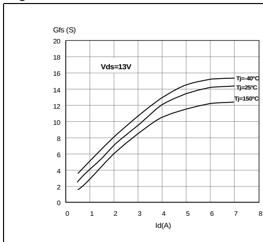
Figure 25. Transconductance
