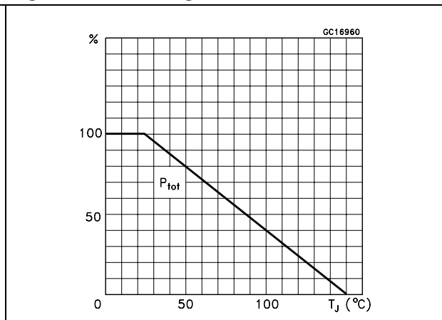
Figure 24. Derating curve
