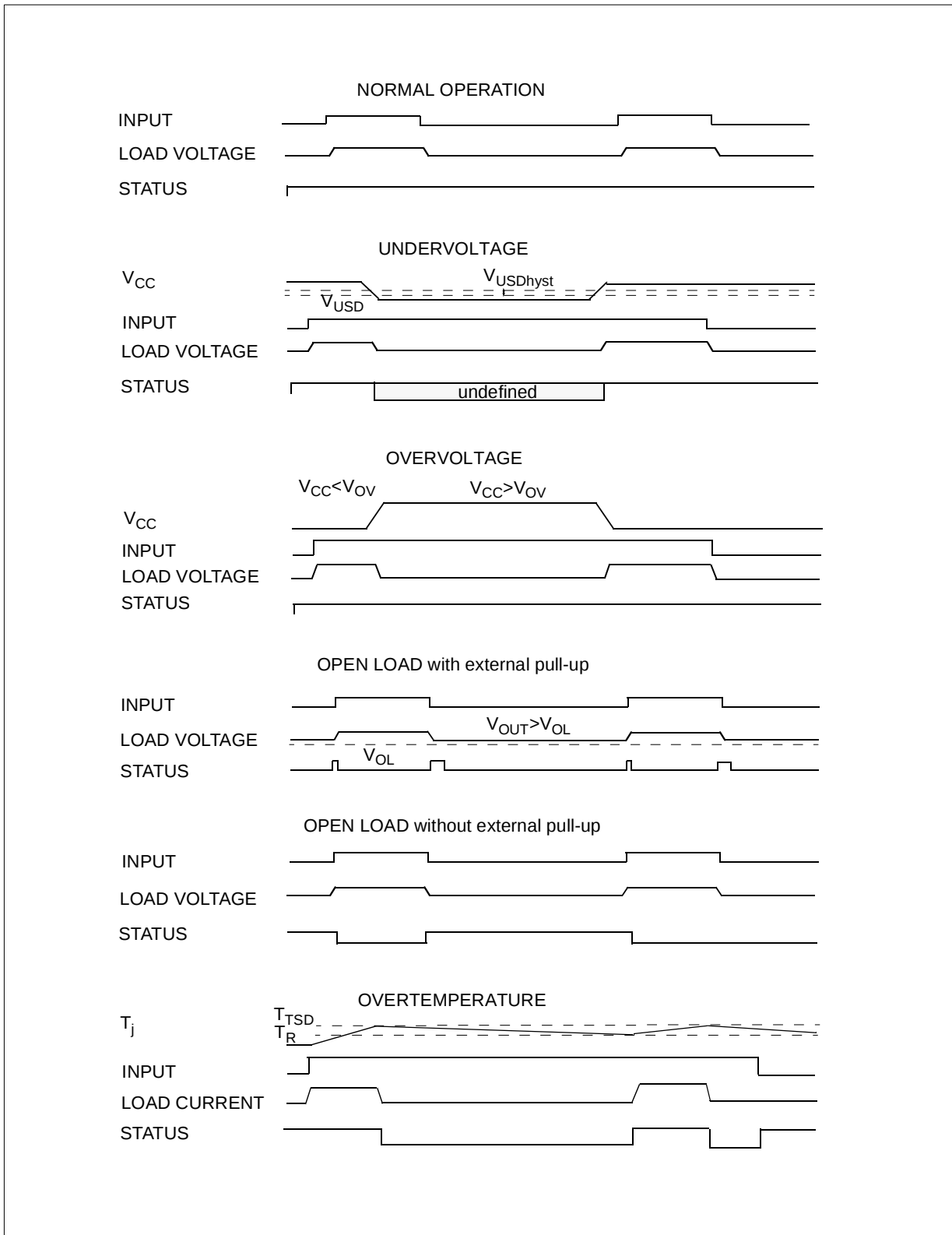
Figure 1: Waveforms
